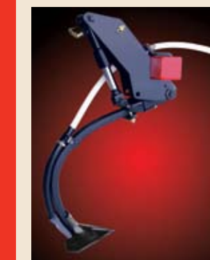
Lifting linkage prevents gouging and ridging for a smoother field finish.
