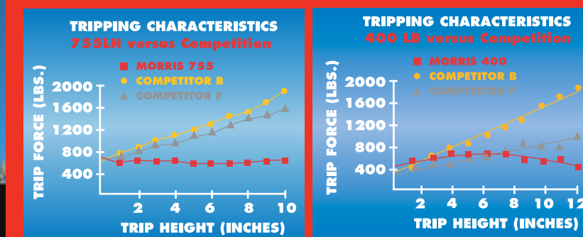
The unique tripping characteristic reduces stress on the trip components and frame members.
